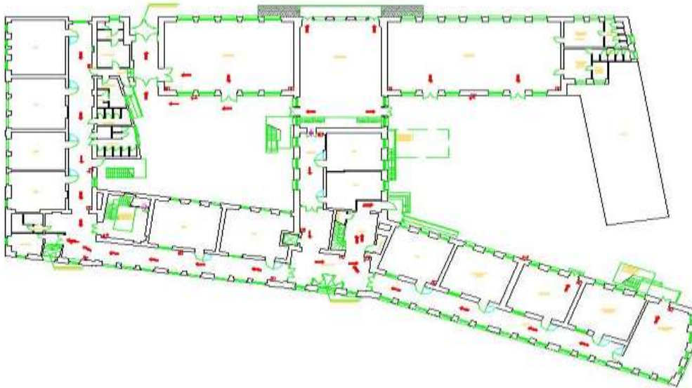
PIANO TERRA
